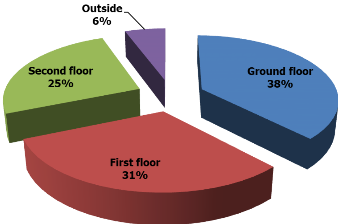
Figure 5: Energy consumed by Lights floor wise
