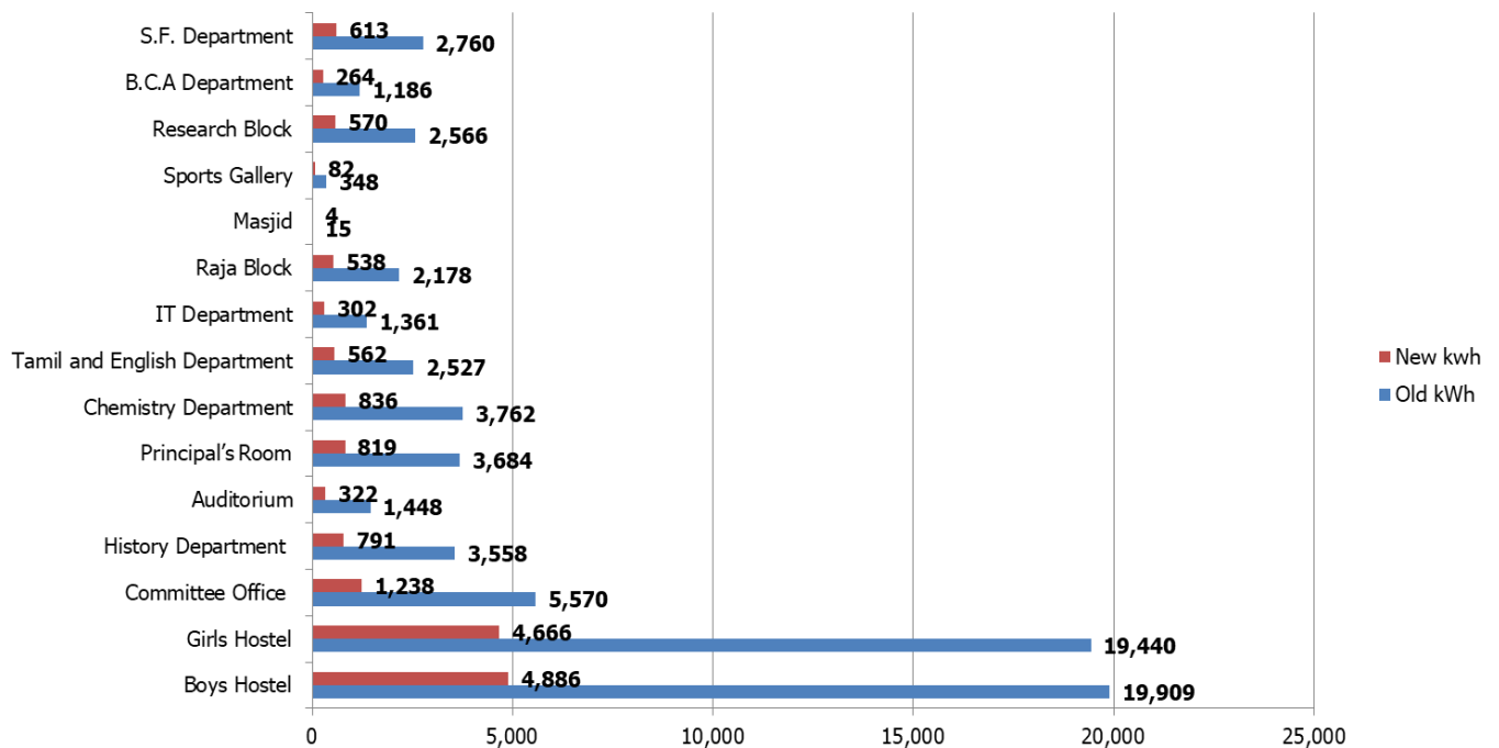
Figure 18: Analysis of current Non-LED and new LED Lights
